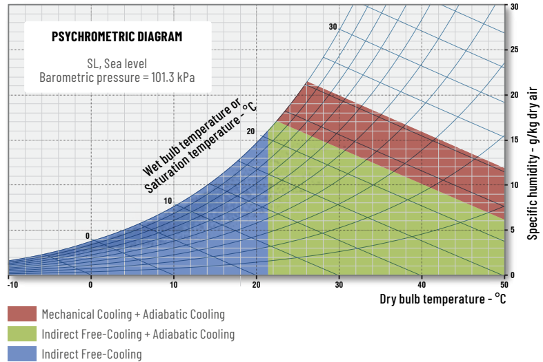
Example of use for a 1 MW Data Center (Redundancy N+1) in Amsterdam at 36°C -25%; Air temp. 24°C; Max air temp. in 26°C
