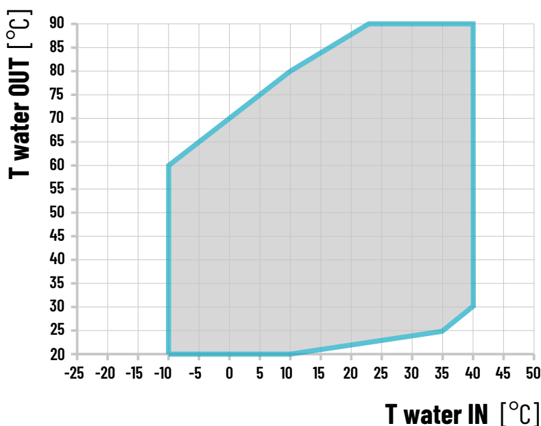
XVA K operating limits - heating
